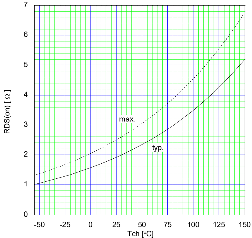
Drain-Source On-state Resistance R_{DS(on)}=f(T_{ch}):I_D=3A, V_{GS}=10V
